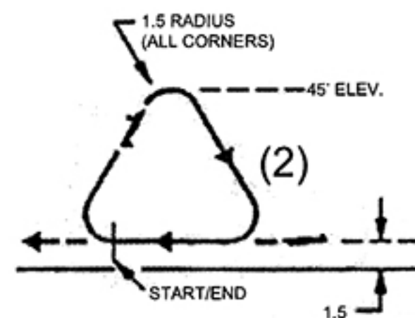
INSIDE TRIANGULAR LOOPS
